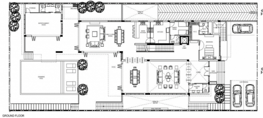
GROUND FLOOR
